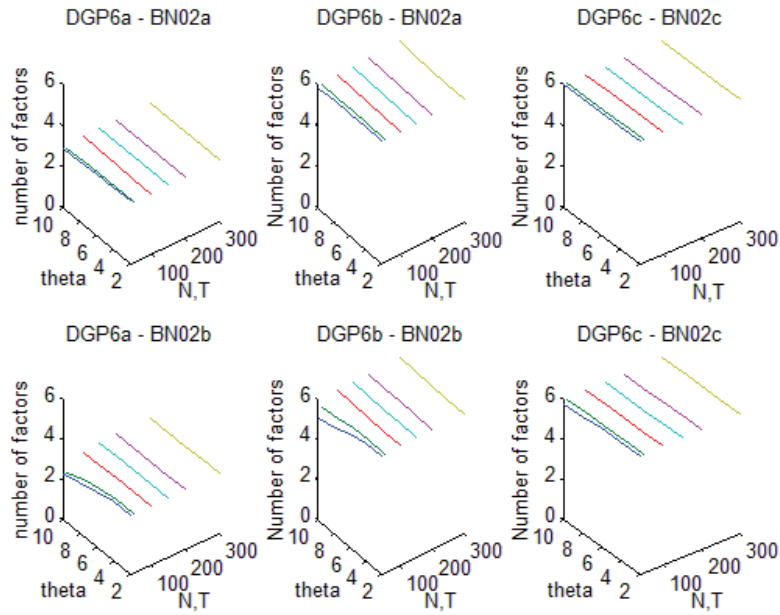
Figure 1: DGP6a: Estimation of number of factors
