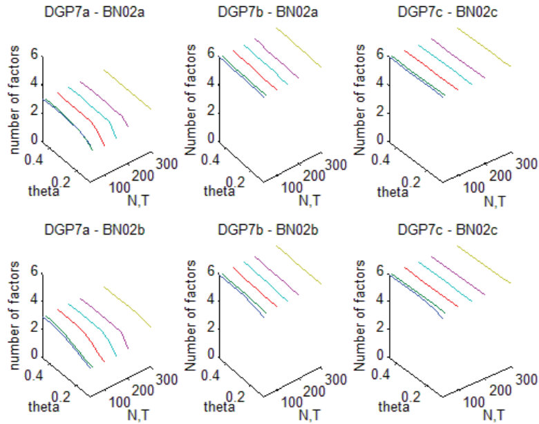
Figure 5: DGP7a: Estimation of number of factors
