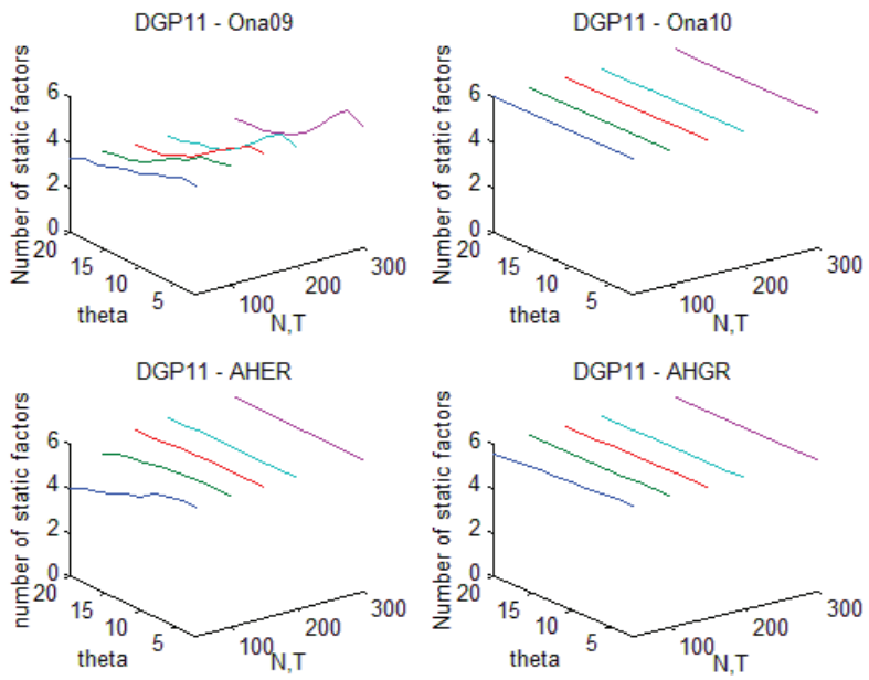
Figure 14: DGP11b: Estimation of number of static factors
