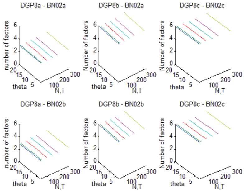
Figure 9: DGP8a: Estimation of number of factors
