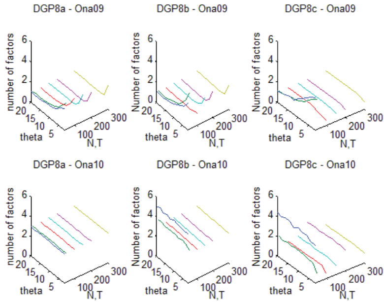
Figure 11: DGP8c: Estimation of number of factors
