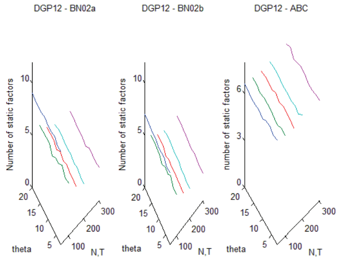
Figure 17: DGP12a: Estimation of number of static factors
