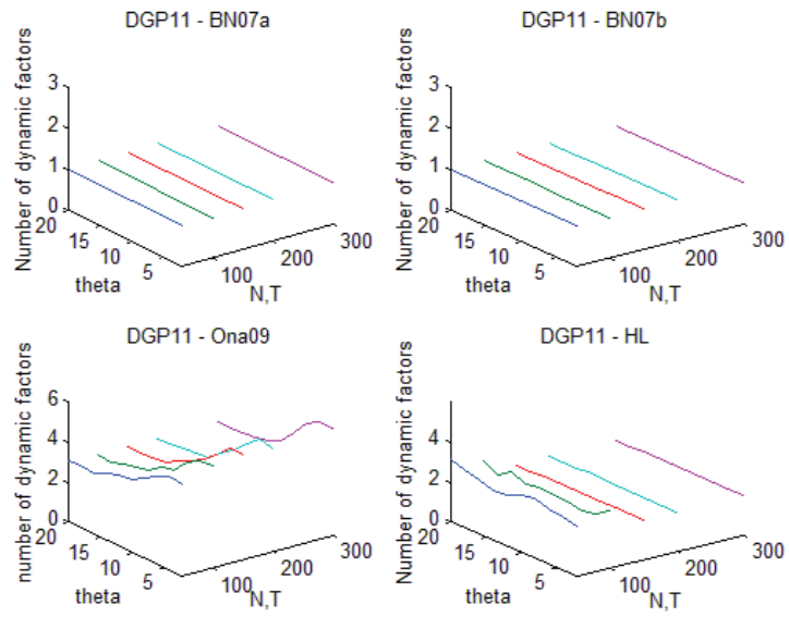
Figure 15: DGP11c: Estimation of number of dynamic factors
