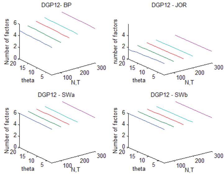
Figure 20: DGP12d: Estimation of number of dynamic factors
