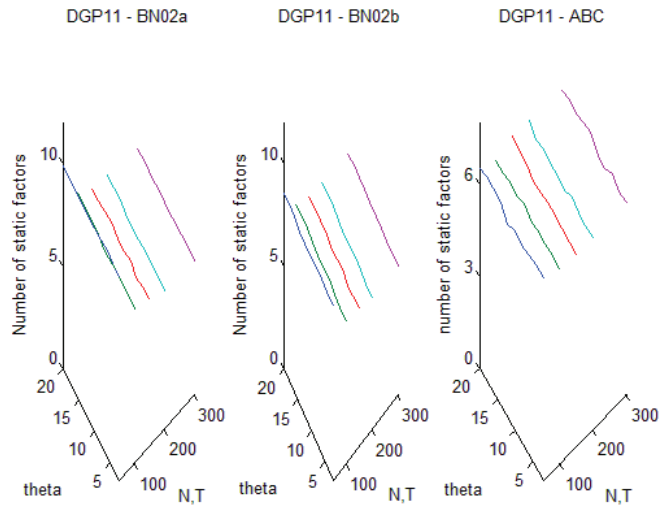
Figure 13: DGP11a: Estimation of number of static factors
