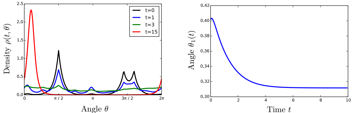
Figure 1: Numerical simulation of the midpoint model on the circle described in Example 2.2. On the left, we have represented the solution x \mapsto \rho(t, x) at various times, as a function of the argument of x , that is \theta = \arg(x) \in [0, 2\pi) . On the right, we have represented the argument \theta_1(t) of the center of mass \int_{x \in \mathbb{S}^1 \subset \mathbb{R}^2} x \rho(t, x) dx , as a function of the time t . This numerical simulation is based on a finite difference scheme.
