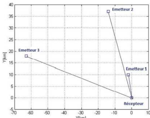
Fig. 4: Positions of the illuminators and the PCL receiver.
