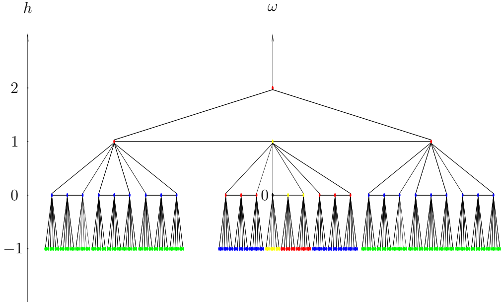
FIGURE 1. Spheres in the upper-half space of (\mathbb{Z}/4\mathbb{Z})^{*4}
