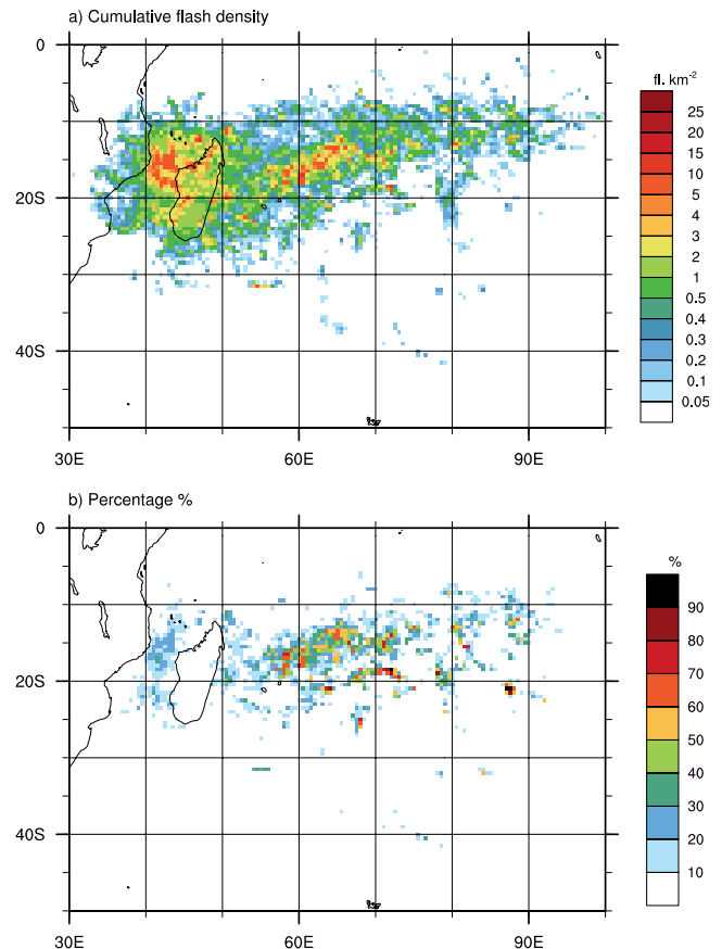
Fig. 3. Impact of tropical storms on the global lightning activity in the SWIO between cyclonic seasons 2005/2006 and 2010/2011. (a) Cumulative flash density (fl km ^{-2} ) associated with TSs, and (b) contribution (%) of lightning generated by TSs.
