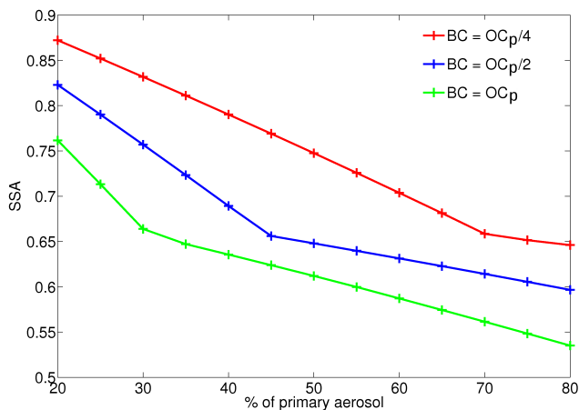
Fig. 3. Single scattering albedo at the 550 \text{ nm} wavelength versus percentage of primary aerosol for 3 different core compositions with a median radius of 0.15 \mu\text{m} and a geometric standard deviation of 1.65 .
