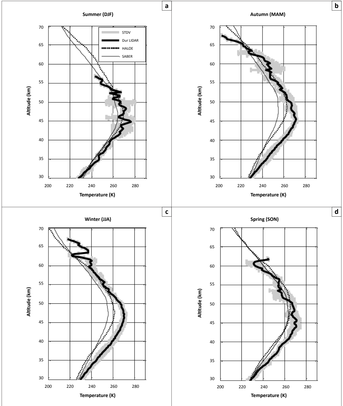
FIGURE 6: Seasonal mean temperature profiles obtained from the Durban LIDAR and the HALOE and SABER satellites for (a) summer (December–February), (b) autumn (March–May), (c) winter (June–August) and (d) spring (September–November).
