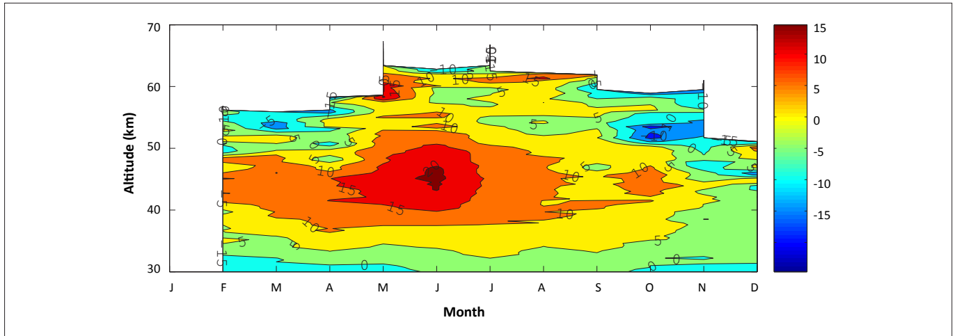
FIGURE 3: Contour plots of temperature differences between the data obtained by the Durban LIDAR and the SABER satellite.
