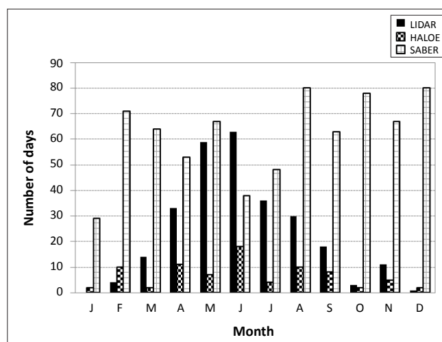
FIGURE 1: A comparison of the monthly distribution of data obtained by the Durban LIDAR and the HALOE and SABER satellites.
