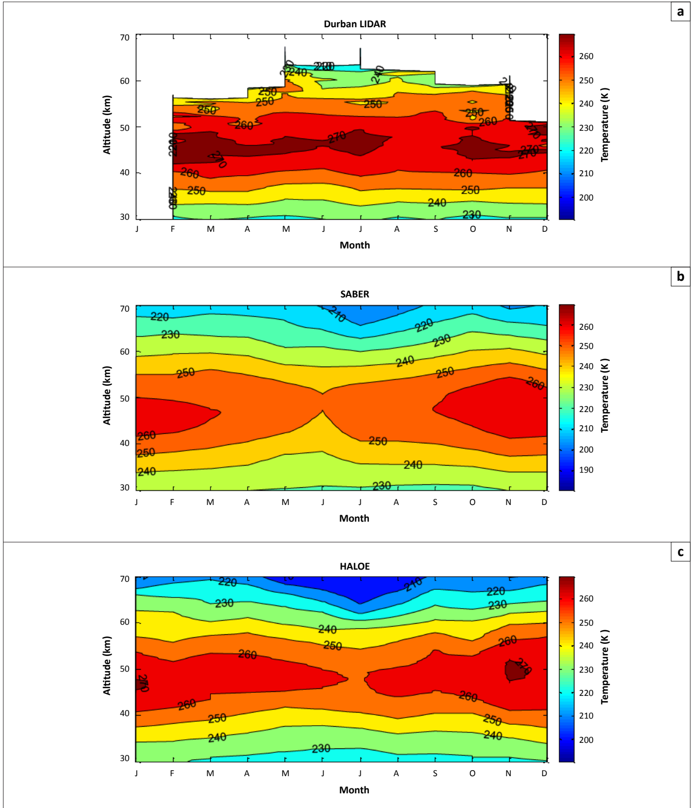
FIGURE 2: Contour plots of monthly climatological temperature variations with altitude (in kilometres) over Durban obtained by the (a) Durban LIDAR, (b) SABER satellite and (c) HALOE satellite.
