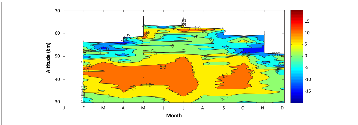
FIGURE 4: Contour plots of temperature differences between the data obtained by the Durban LIDAR and the HALOE satellite.
