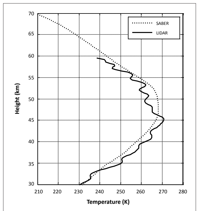
FIGURE 5: A quasi-simultaneous height profile of the temperature observed by the Durban LIDAR and the SABER satellite over Durban, South Africa for the night of 27–28 November 2002.
