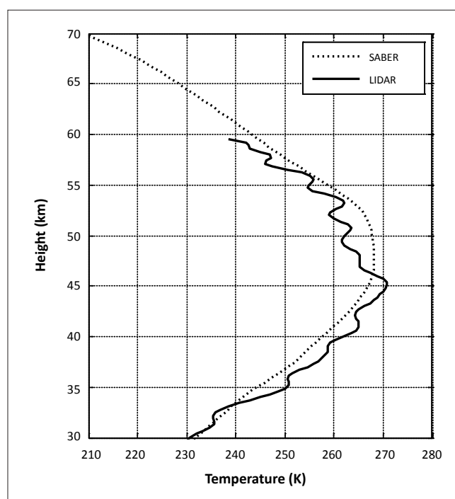
FIGURE 5: A quasi-simultaneous height profile of the temperature observed by the Durban LIDAR and the SABER satellite over Durban, South Africa for the night of 27–28 November 2002.
