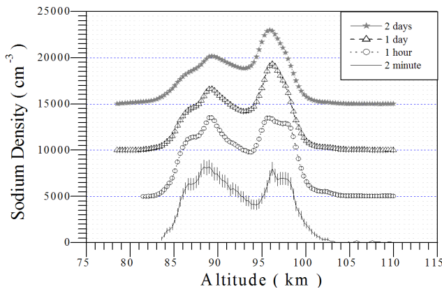
Fig. 2. Height profile of sodium density averaged over different time scales. The vertical bar represents the statistical error in the retrieved Na concentration. The profiles are vertically offset by 5 \times 10^3 .
