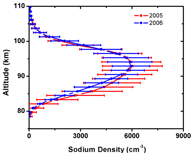
Fig. 10. Annual mean sodium density profiles for the year 2005 and 2006.
