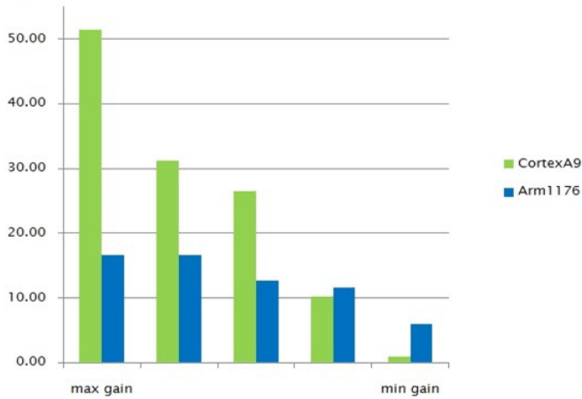
Fig. 5. DSF energy savings for H.264 encoder
