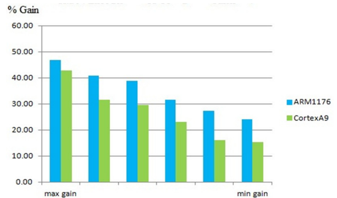
Fig. 8. AsDPM energy savings for H.264 encoder
