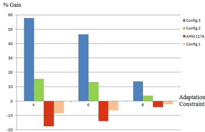
Fig. 2. Energy gains of DVFS video strategy
