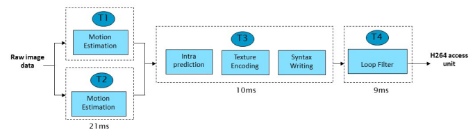
Fig. 4. H.264 encoder block diagram
