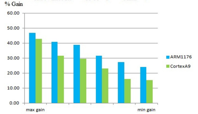
Figure 8: AsDPM energy savings for H.264 encoder
