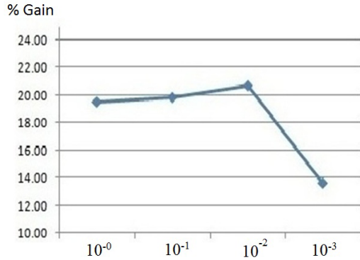
Figure 6: Energy gain vs. time granularity of tasks (sec)
