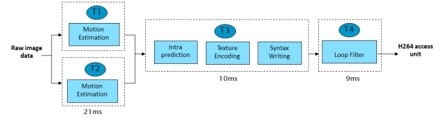
Figure 4: H.264 encoder block diagram
