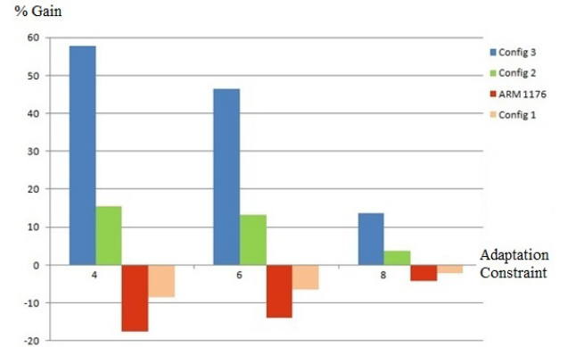
Figure 2: Energy gains of DVFS video strategy
