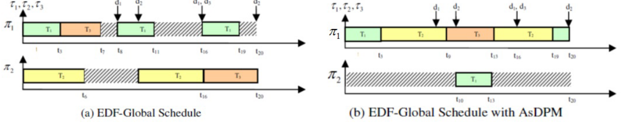
Figure 7: AsDPM scheduling principle
