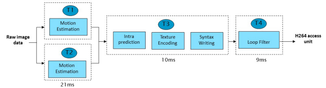
Fig. 4 H.264 encoder block diagram
