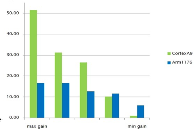
Fig. 5 DSF energy savings for H.264 encoder
