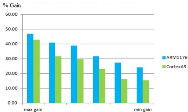
Fig. 8 AsDPM energy savings for H.264 encoder
