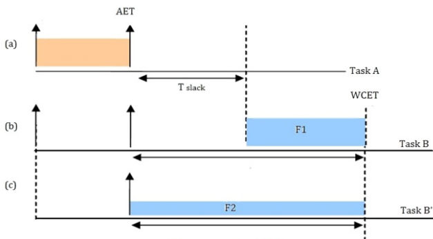
Fig. 3 DSF scheduling principle
