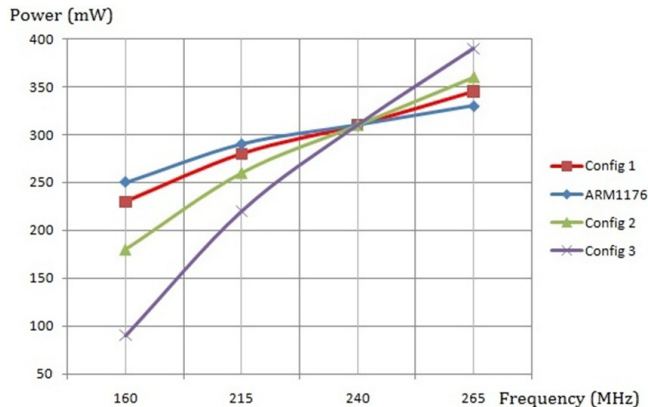
Fig. 1 QEMU operating point configurations
