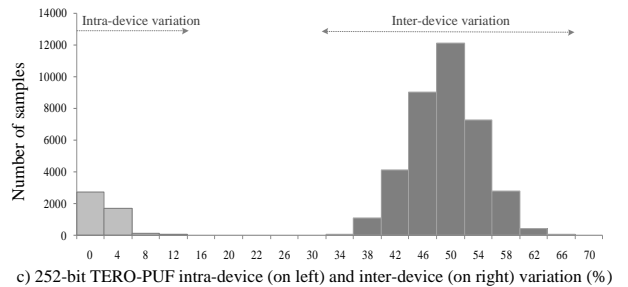
Fig. 6 TERO-PUF intra- (left) and inter-device (right) variation.
