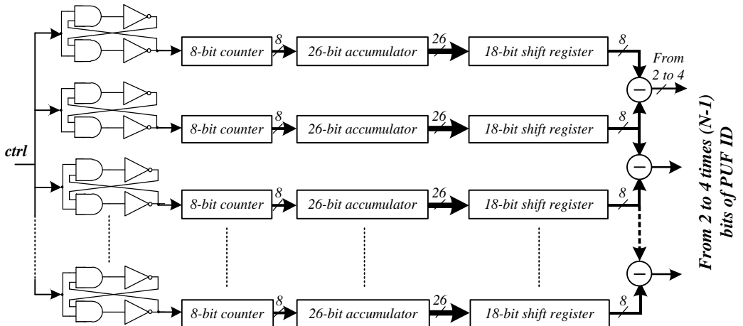
Fig. 3. TERO-PUF architecture.
