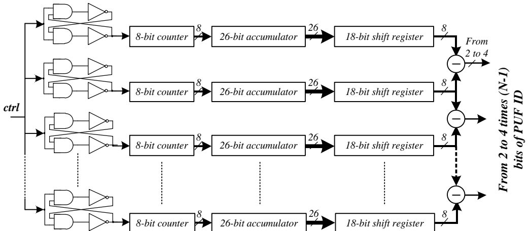
Fig. 3. TERO-PUF architecture.
