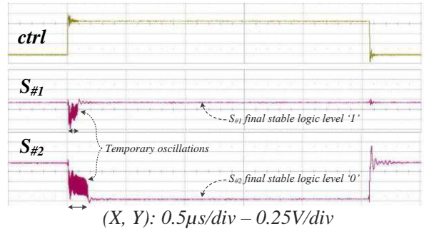
Fig. 2. Electrical behavior of the two TERO loops
