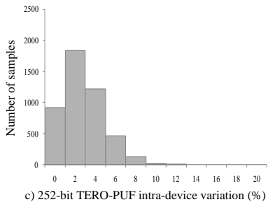
Fig. 5 TERO-PUF intra-device variation.
