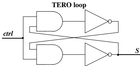
Fig. 1. TERO loop structure.
