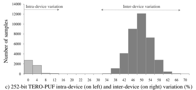
Fig. 6 TERO-PUF intra- (left) and inter-device (right) variation.
