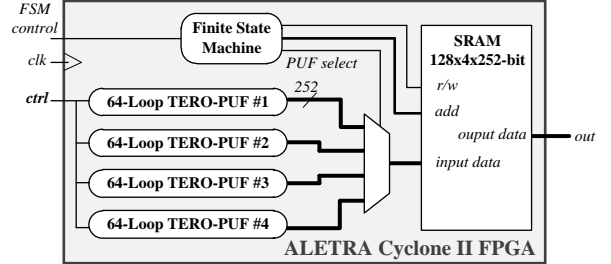
Fig. 4. FPGA Implementation of four 64-loop TERO-PUFs.
