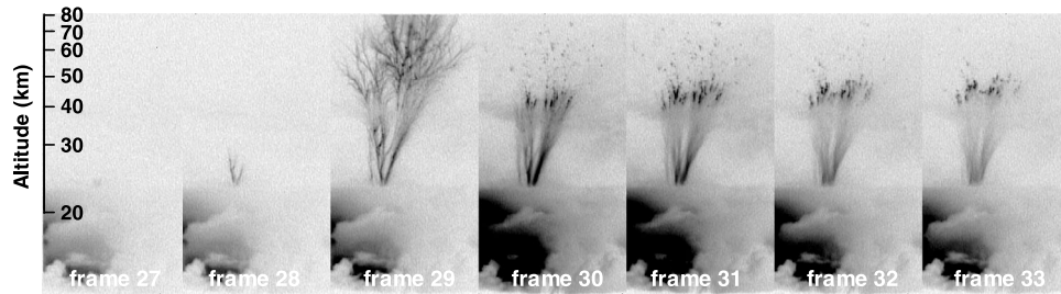
Figure 9. Seven successive de-interlaced frames in inverted color from the video imagery of GJ4, t = 434.2\text{--}551.1 ms, leading jet/beginning of the trailing jet with beads. The time reference t = 0 (frame 1) corresponds to the first cloud brightening of the event. The vertical scale is calculated at the distance of the GJ by taking into account the perspective effect and is not valid at the distance of the cloud edge.
