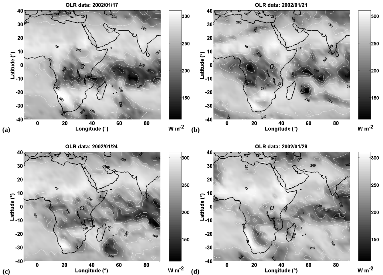
Fig. 7. Maps of 2.5^{\circ} – 2.5^{\circ} gridded NOAA Interpolated Outgoing Longwave Radiation (OLR) at longitudes between -10^{\circ} W and 90^{\circ} E and at latitudes between 40^{\circ} N and -40^{\circ} S: on (a) 17 January, (b) 21 January, (c) 24 January and (d) 28 January 2002.
