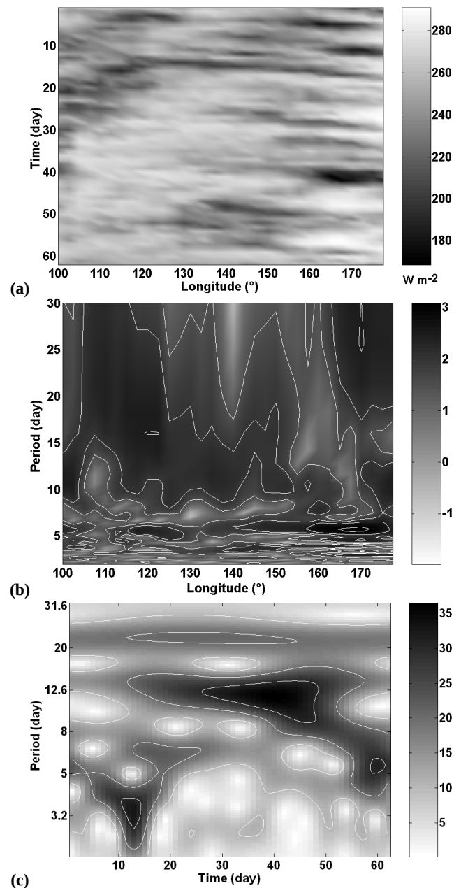
Fig. 11. (a) Hovmöller diagram (time versus longitude) of 2.5^{\circ} – 2.5^{\circ} gridded NOAA Interpolated MJO filtered OLR data averaged over latitudes between 0^{\circ} N and 20^{\circ} N for longitudes between 100^{\circ} E and 177.5^{\circ} E and from 1 December 2001 to 31 January 2002, (b) Period-longitude distribution of Fast Fourier Transform spectral density in base-10 logarithmic scale and (c) Period-time diagram of modulus of continuous complex Morlet transform coefficients (5 octaves and 30 voices). OLR data is filtered by using a fourth-order polynomial fit.
