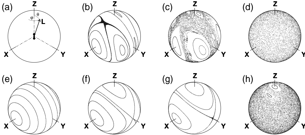
Fig. 1 – Poincaré surfaces of section in the molecular frame. (a) defines the angles \theta and \varphi for a given position of L on the sphere. The core axis is along OZ and N along OX . (e) shows the k=0 , no coupling situation, valid for all values of T_e and T_0 ; one sees only the free apparent rotation of L around the core angular momentum N , describing circles. On a given circle, the modulus N is constant, but it varies from circle to circle. (b)-(d) and (f)-(h): generic case (top row) and resonant ( T_e = T_0 ) case (bottom row) for increasing coupling. (b) and (f): k = 0.25 , (c) and (g): k = 0.5 , (d) and (h): k = 10 . Note that in the generic case, circles (torii in whole phase space) which correspond to low rational values of the returning times of electron and core open resonant islands: values 2 and 4 appear clearly in (b). Chaos appears along the corresponding unstable manifolds and invades rapidly the whole phase space until the last islands of regularity disappear [(d)]. In the resonant case a very large couple of resonance islands appears around the \pm OZ axis (the top one is visible in (f)-(h)), with a separatrix starting from the \pm OY axis.
