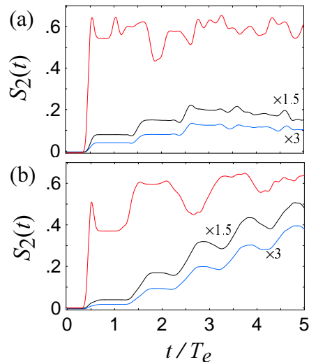
Fig. 3 – Short time variation of the linear entropy for different values of the coupling strength; t is given in units of the Kepler period T_e . (a) Generic phase-space, from top to bottom k = 10 (red), 0.5 (black) and 0.25 (blue). The k = 0.25 ( k = 0.5 ) curve is multiplied by a factor 3 (1.5). (b) Same as (a) for the resonant case T_e = T_0 .
