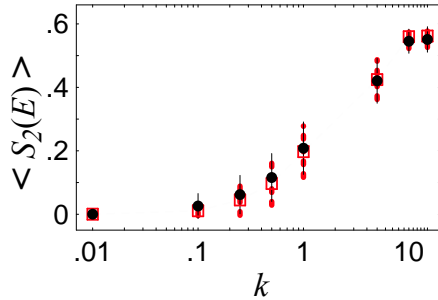
Fig. 2 – Average linear entropy for generic (red/gray boxes) and resonant (black dots) states ( T_e = T_0 ), shown for different values of k . The rms is also shown as red dashed (generic) and solid (resonant) error bars.
