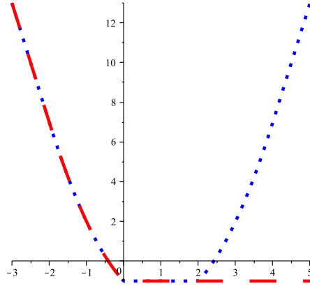
Figure 4: The graphs of the Hamiltonian p \mapsto \overline{H}_i(0, p) and of p \mapsto \overline{H}_i^+(0, p) coincide for p \leq \bar{p}_i , and \overline{H}_i^+(0, p) = \Lambda_i^0 for p \geq \bar{p}_i . In the example, \underline{p}_i = 0 and \bar{p}_i = 2 .
