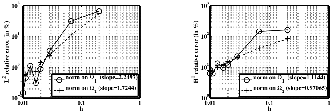
Figure 6: Convergence curves in 2D for the method \theta = 1 , with \gamma_0 = 1/200 and P_1 finite elements for the relative L^2 -norm of the error (on the left) and the relative H^1 -norm of the error (on the right).
