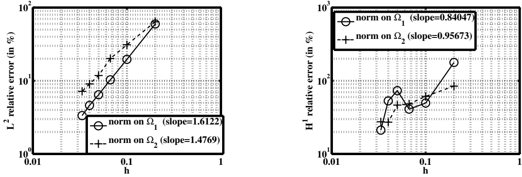
Figure 14: Convergence curves in 3D for the method \theta = 1 , with \gamma_0 = 1/100 and P1 finite elements for the relative L^2 -norm of the error (on the left) and the relative H^1 -norm of the error (on the right).
