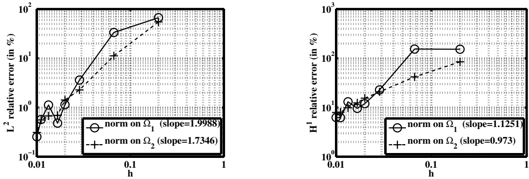
Figure 8: Convergence curves in 2D for the method \theta = -1 , with \gamma_0 = 1/200 and P_1 finite elements for the relative L^2 -norm of the error (on the left) and the relative H^1 -norm of the error (on the right).
