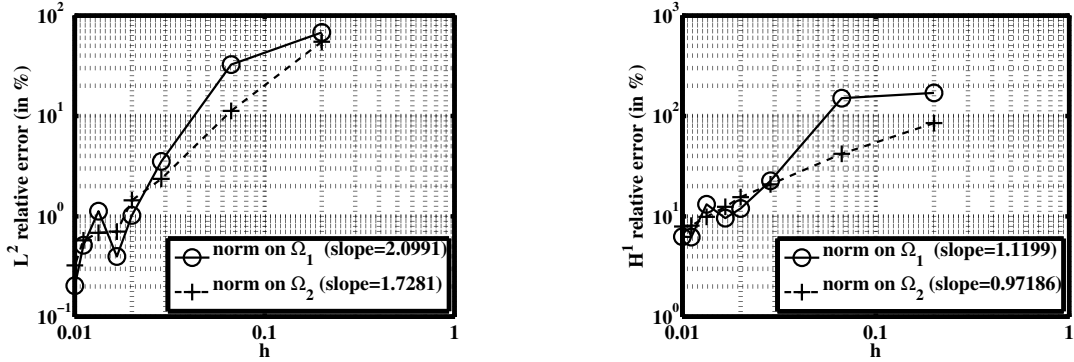
Figure 7: Convergence curves in 2D for the method \theta = 0 , with \gamma_0 = 1/200 and P_1 finite elements for the relative L^2 -norm of the error (on the left) and the relative H^1 -norm of the error (on the right).
