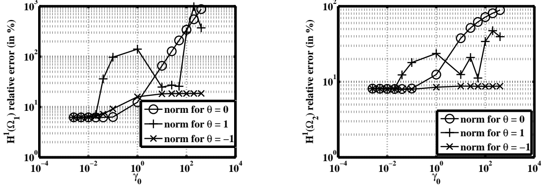
Figure 12: Influence of \gamma_0 on the relative H^1 -norm of the error on \Omega_1 (on the left) and on \Omega_2 (on the right) in 2D for h = 1/90 and P_1 elements.
