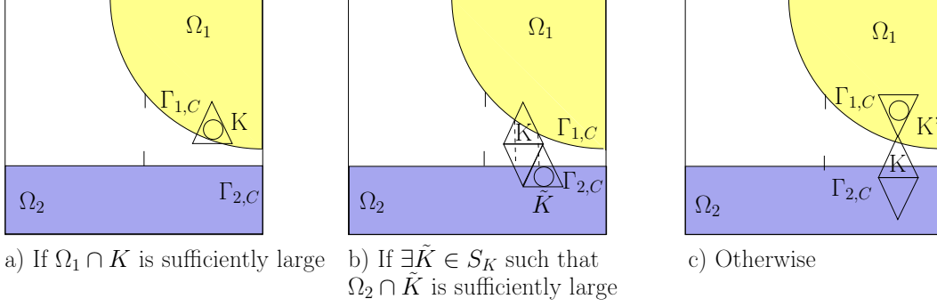
Figure 3: The different cases for the definition of R_{\hat{\rho}} .
