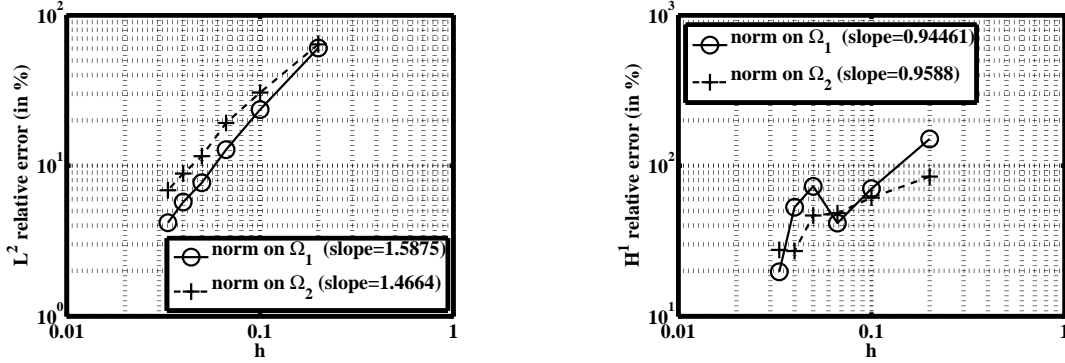
Figure 16: Convergence curves in 3D for the method \theta = -1 , with \gamma_0 = 1/100 and P1 finite elements for the relative L^2 -norm of the error (on the left) and the relative H^1 -norm of the error (on the right).
