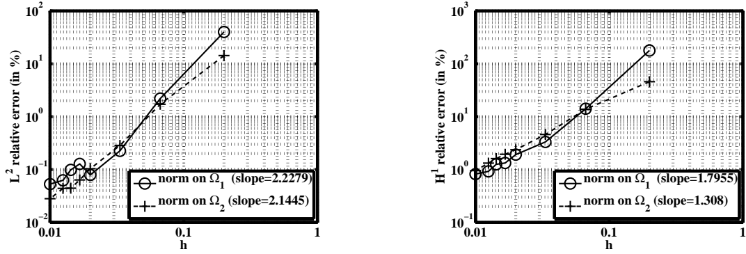
Figure 10: Convergence curves in 2D for the method \theta = 0 , with \gamma_0 = 1/200 and P2 finite elements for the relative L^2 -norm of the error (on the left) and the relative H^1 -norm of the error (on the right).
