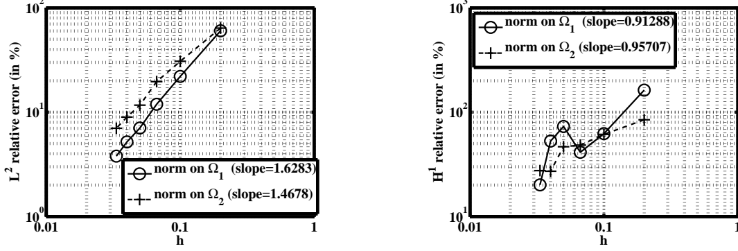
Figure 15: Convergence curves in 3D for the method \theta = 0 , with \gamma_0 = 1/100 and P1 finite elements for the relative L^2 -norm of the error (on the left) and the relative H^1 -norm of the error (on the right).
