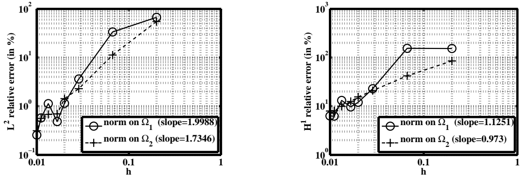
Figure 8: Convergence curves in 2D for the method \theta = -1 , with \gamma_0 = 1/200 and P1 finite elements for the relative L^2 -norm of the error (on the left) and the relative H^1 -norm of the error (on the right).
