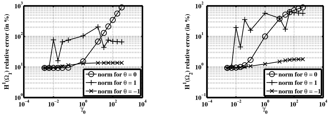
Figure 13: Influence of \gamma_0 on the relative H^1 -norm of the error on \Omega_1 (on the left) and on \Omega_2 (on the right) in 2D for h = 1/90 and P_2 elements.
