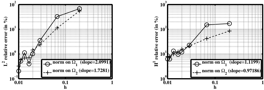
Figure 7: Convergence curves in 2D for the method \theta = 0 , with \gamma_0 = 1/200 and P1 finite elements for the relative L^2 -norm of the error (on the left) and the relative H^1 -norm of the error (on the right).
