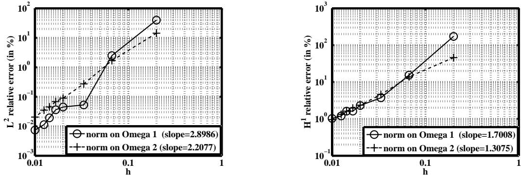
Figure 11: Convergence curves in 2D for the method \theta = -1 , with \gamma_0 = 1/200 and P2 finite elements for the relative L^2 -norm of the error (on the left) and the relative H^1 -norm of the error (on the right).
