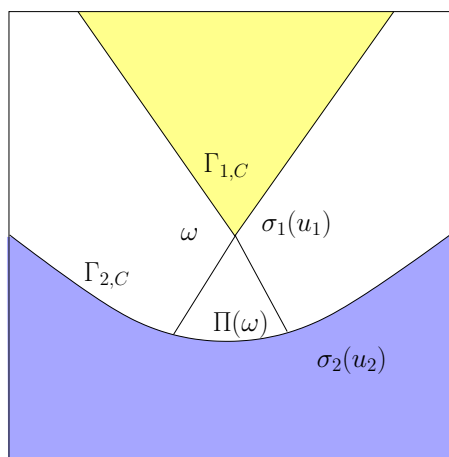
Figure 17: Example of non regular situation on \Gamma_{1,C} .
