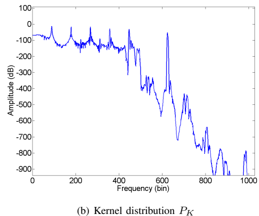
Figure 2. Scale-invariant PLCA: Kernel and impulse.
