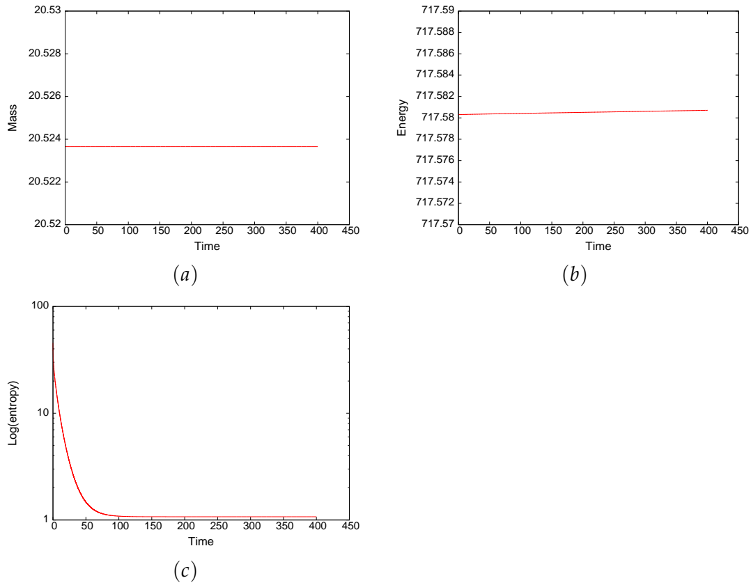
Figure 5: Evolution mass (a), energy (b) and entropy(c) in the case of \zeta_{\max} = 20 with 64 points for bi-Maxwellian initial data.
