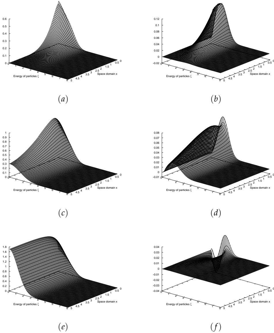
Figure 9: Description of moments F^0 and F^1 with respect to the energy \zeta at time t = 0.015 (a) and (b), at time t = 0.15 (c) and (d) and at time t = 100 (e) and (f) in the case of \zeta_{\max} = 8 with 64 points and x_{\max} = 5 with 100 points for electron beam data.
