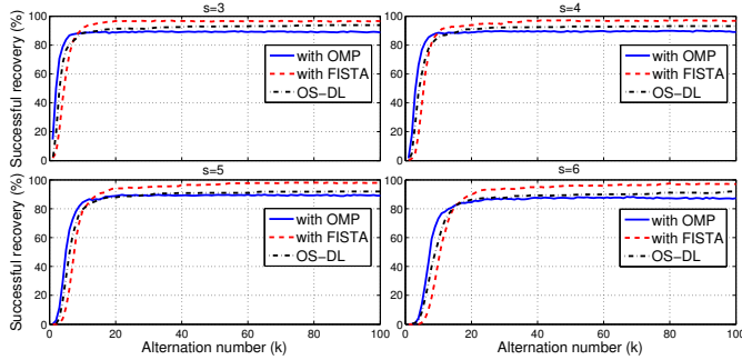
Fig. 4. Convergence behaviour of OS-DL and APru-DL with (Batch) OMP and (Batch) FISTA as the sparse approximation stage. The setup is the same as in Fig. 3.
