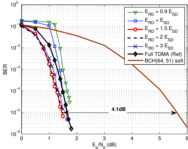
Fig. 7. BER versus E_b/N_0 of the CDMA-TDMA cooperation, BPSK, AWGN channel, E_b excludes the energy from relay-destination channel.
