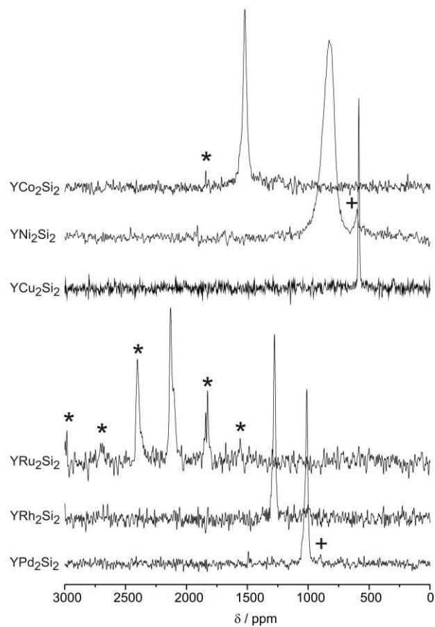
Fig. 5. 24.5 MHz solid state NMR spectra of the series of YT_2Si_2 ( T = Co, Ni, Cu, Ru, Rh, Pd ) silicides at room temperature (from top to bottom). Impurities and spinning sidebands are marked by crosses and asterisks, respectively.
