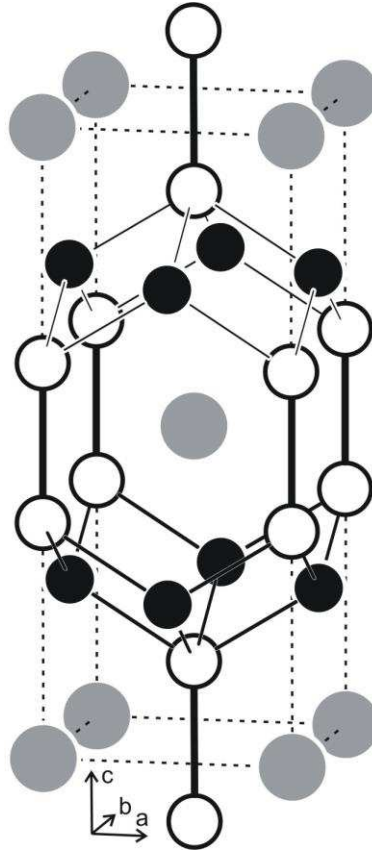
Fig. 1. The crystal structure of the silicides \text{YT}_2\text{Si}_2 . Yttrium, transition metal, and silicon atoms are drawn as medium grey, black filled and open circles, respectively. The three-dimensional [\text{T}_2\text{Si}_2] network is emphasized.
