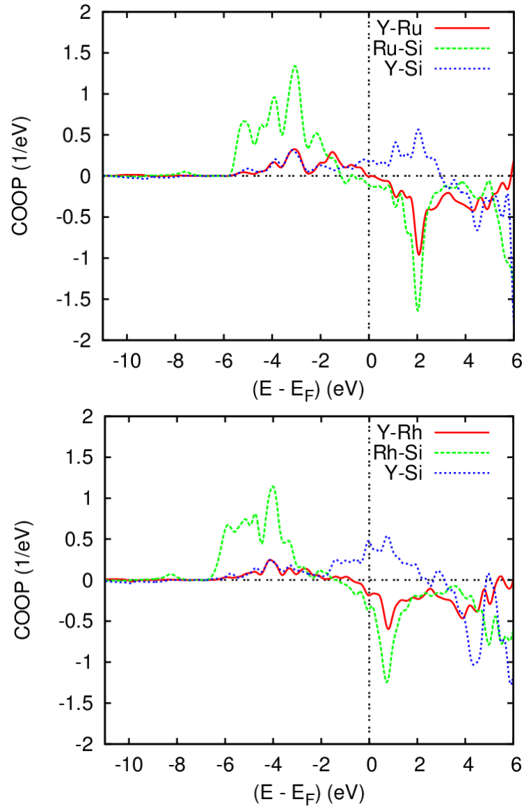
Fig. 4 (color online). Chemical bonding from overlap populations with the COOP criterion for the different interactions in \text{YRu}_2\text{Si}_2 (top) and \text{YRh}_2\text{Si}_2 (bottom).
