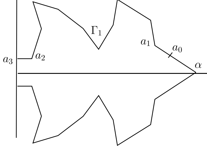
Figure 1: The curve constructed in the proof of Theorem 2.5
