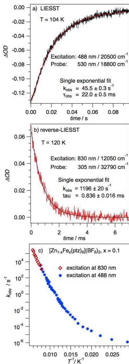
Figure 4. The HS \rightarrow LS relaxation in [\text{Zn}_{1-x}\text{Fe}_x(\text{ptz})_6](\text{BF}_4)_2 , x = 0.1 : a) transient absorption at 530 nm for \lambda_{\text{exc}} = 488 nm at 104 K (LIESST); b) transient absorption at 305 nm for \lambda_{\text{exc}} = 830 nm and 120 K (reverse-LIESST); c) observed relaxation rate constant k_{\text{obs}} = k_{\text{HL}} + k_{\text{LH}} vs. T^{-1} on a logarithmic scale, ( \bullet ) \lambda_{\text{exc}} = 488 nm (taken from Ref. [4]) and ( \blacklozenge ) \lambda_{\text{exc}} = 830 nm.
