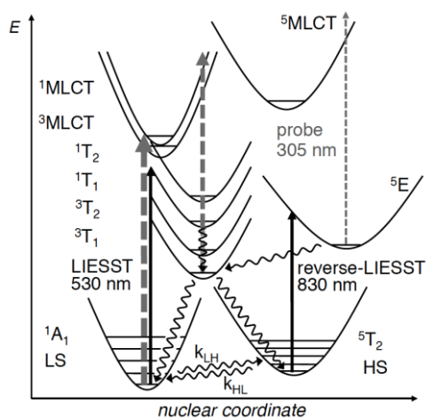
Figure 2. Schematic representation of the electronic structure of iron(II) spin-crossover compounds with only high-energy MLCT states. LIESST ( \lambda_{\text{ex}} = 530 nm) and reverse-LIESST ( \lambda_{\text{ex}} = 830 nm) via the LF states as in [\text{Fe}(\text{ptz})_6](\text{BF}_4)_2 are indicated by curly arrows. The 305 nm probe (---) monitors the MLCT transitions.
