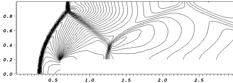
Figure 1: Density order 1 t=3.5
