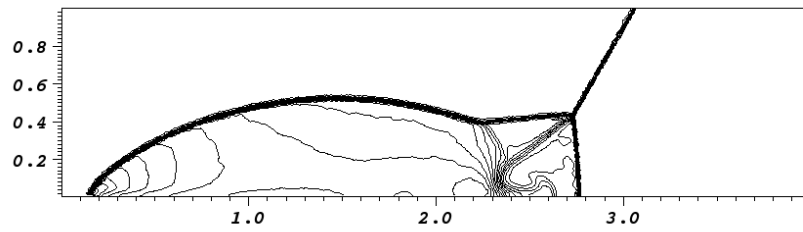
Figure 7: Density order 2 rk2 local T=0.2s
