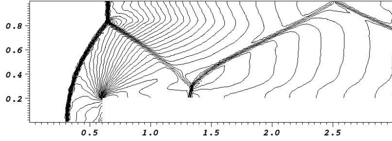
Figure 3: Density order 2 local t=3.5
