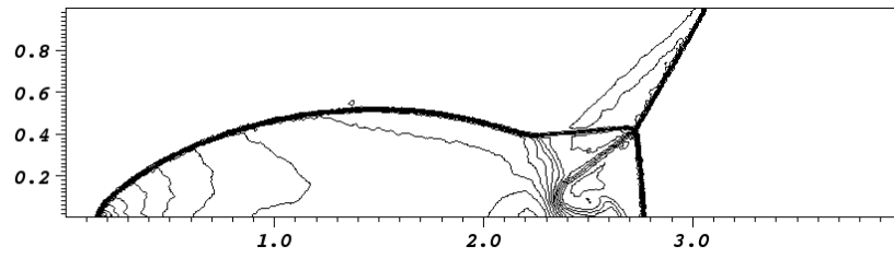
Figure 6: Density order 2 local T=0.2s
