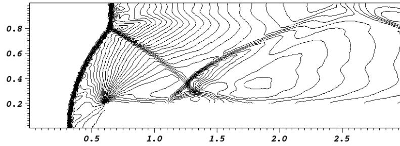
Figure 2: Density order 2 t=3.5
