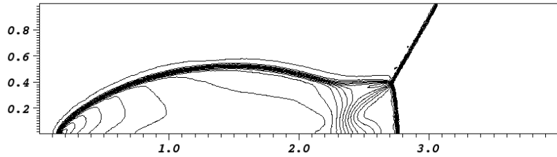
Figure 5: Density order 1 T=0.2s
