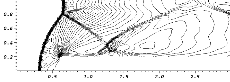
Figure 2: Density order 2 t=3.5
