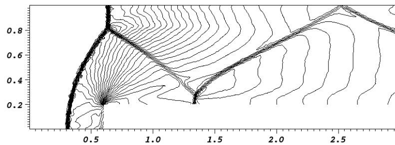
Figure 4: Density order 2 rk2 local t=3.5
