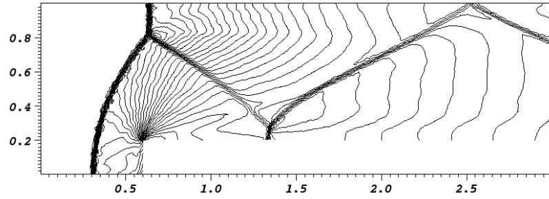
Figure 4: Density order 2 rk2 local t=3.5
