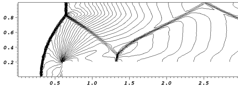
Figure 3: Density order 2 local t=3.5
