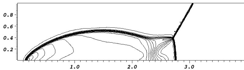
Figure 5: Density order 1 T=0.2s
