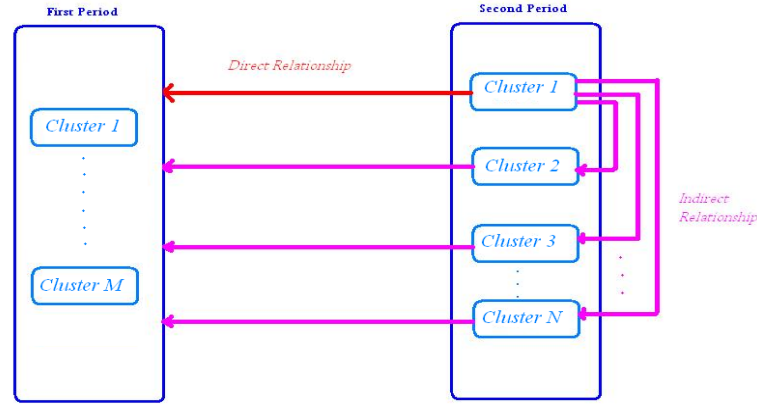
Figure 2: Illustration of the two types of cluster relationships between the two periods
