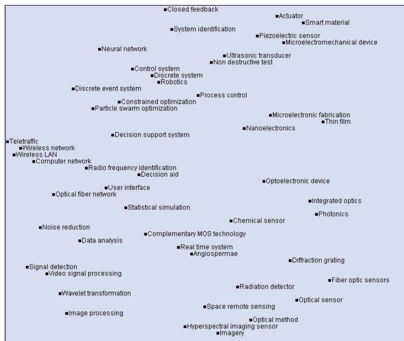
Figure 3: Obtained cluster map for P2
