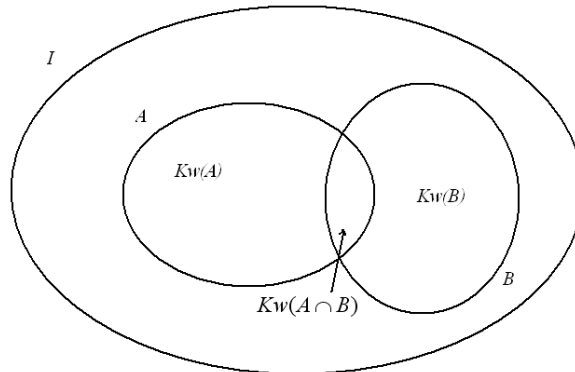
Figure 1: Illustration of A \Rightarrow B
