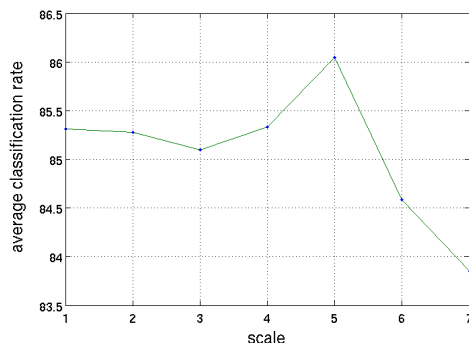
Figure 5: Average classification rate as a function of the descriptors scale using UNN_s .
