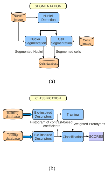
Figure 1: Block diagram of the proposed method for automatic cell classification: (a) cell segmentation step and (b) descriptor extraction and classification process.
