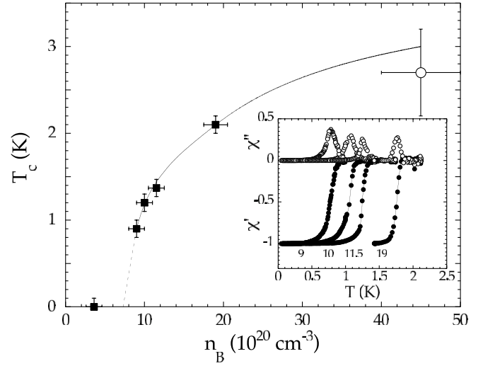
FIG. 2. Dependence of the superconducting transition temperature T_c on the boron concentration n_B : solid squares—this work, open circles—from [1]. The different T_c values were obtained from the onset of the diamagnetic signal (see inset for the real (solid symbols) and imaginary (open symbols) parts of the magnetic susceptibility).
