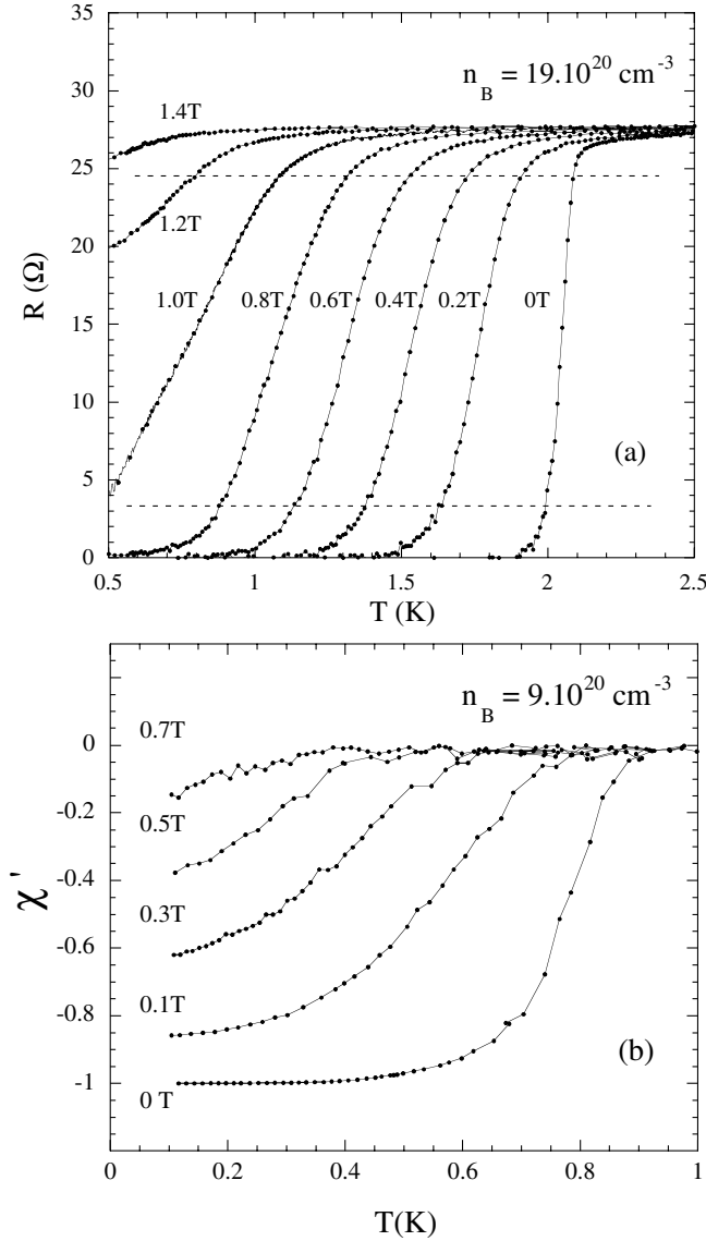
FIG. 3. (a) Temperature dependence of the electrical resistance at indicated magnetic fields for the film with n_B = 19 \times 10^{20} \text{ at. cm}^{-3} . The dashed lines correspond to the two criteria used for the determination of H_{c2} (see Fig. 4), i.e., R/R_N = 90\% and 10\% ( R_N being the normal state resistance). (b) Temperature dependence of the real part of the magnetic susceptibility at indicated magnetic fields for the film with n_B = 9 \times 10^{20} \text{ at. cm}^{-3} . H_{c2} has been deduced from the onset of the diamagnetic signal.
