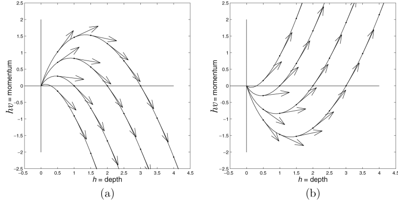
Figure 2.9: (a) Integral curves of the eigenvector r_1 for the shallow water equations. The eigenvector r_1(q) evaluated at any point on a curve is tangent to the curve at that point. (b) Integrals curves for r_2 (From Ref. [5])
