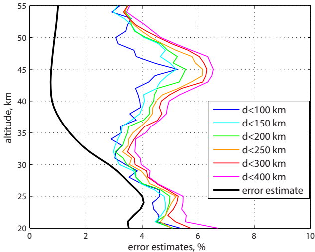
Figure B1. Color lines: experimental precision estimates \frac{s_{12}}{\sqrt{2}} for different separation distances; black line: mean error estimate. GOMOS self-collimations of star S30 occultations close to the North Pole in 2007–2008 are used.
