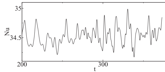
FIG. 8. Gas radiation case – Ra = 3 \times 10^7 . Instantaneous Nusselt number Nu(x = 0.5, t) averaged over y and z directions.
