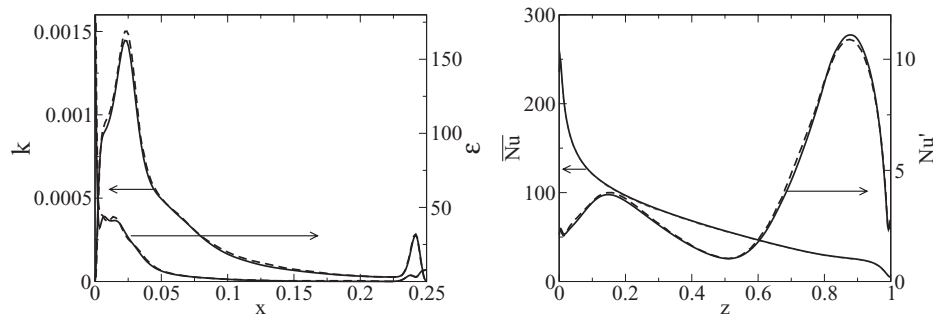
FIG. 2. Left: turbulent kinetic energy k = 0.5\overline{u'_i u'_i} and turbulent kinetic dissipation \epsilon = \overline{(\partial u'_i / \partial x_j)(\partial u'_i / \partial x_j)} at z = 0.8 . Right: mean Nusselt number and its standard deviation Nu' on the hot wall x = 0 . Our results in solid lines are compared to those of Trias et al. 38,40 in dashed lines.
