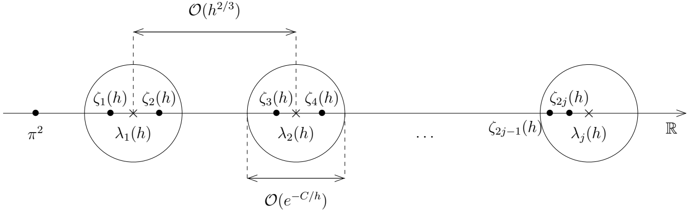
Figure 4: Repartition of \mathfrak{S}(\mathcal{L}(h)) around \mathfrak{S}(\mathcal{L}(h))
