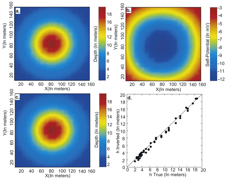
Figure 2. Synthetic test. (a) Synthetic case showing a Gaussian depression of the water table. (b) Distribution of the resulting self-potentials at the ground surface (with c^l = -4 mV/m and h_0 = 2 m). (c) Inverted result of the water table (RMS error 1.15%). (d) True depth of the water table versus the inverted depth of the water table.
