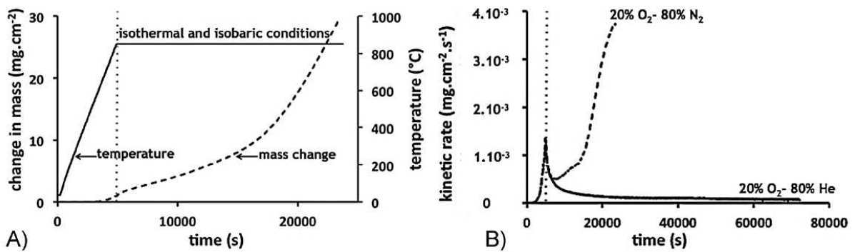
Figure 2 : (A) mass change in 20% O 2 -80% N 2 as a function of time (hyphenated curve); (B) kinetic rate as a function of time in 20% O 2 -80% N 2 (hyphenated curve) and in 20% O 2 -80% He (full curve)
