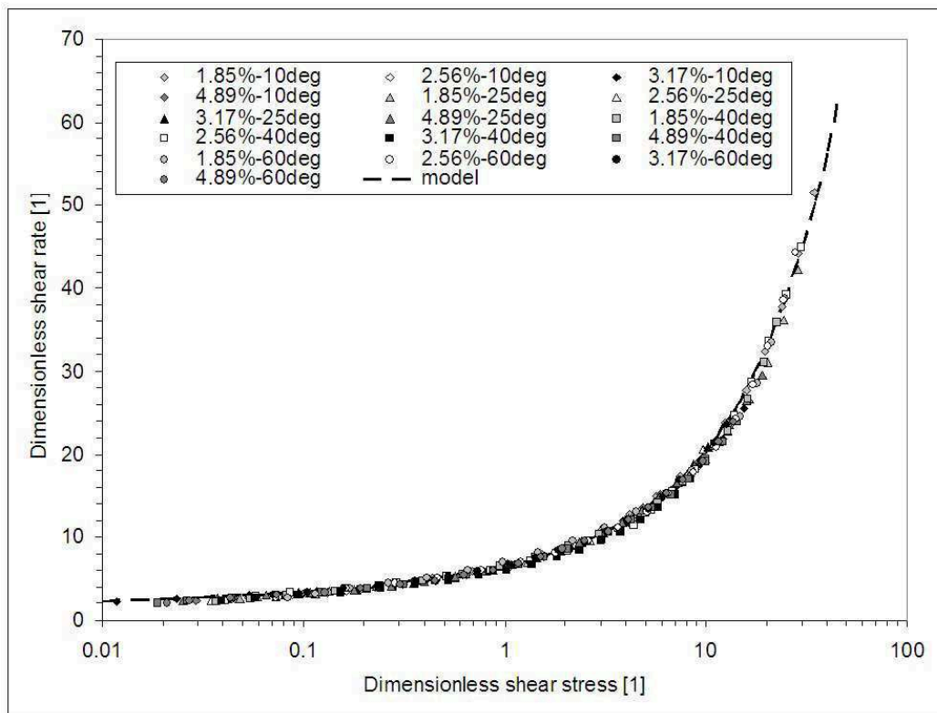
Figure 4: Dimensionless flow curves of the digested sludge at different solids concentration and temperature. The dotted line represents the model of Equation (2) with the following parameters:
