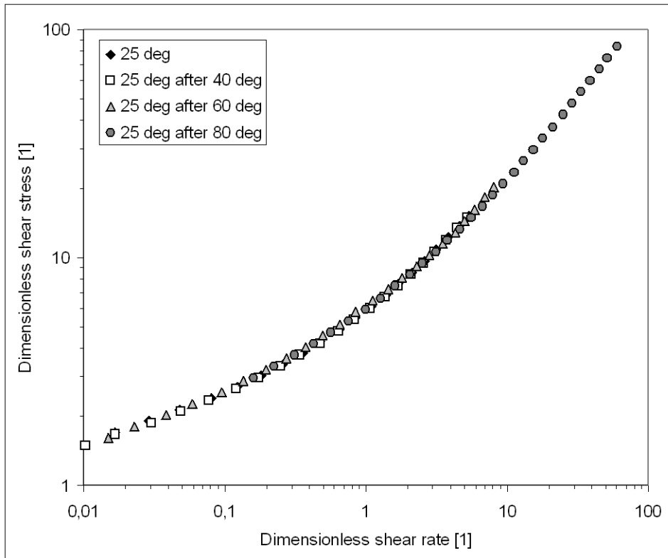
Figure 10: Dimensionless flow curve of the 3.2% digested sludge at 25°C after being heated to 40. 60 and 80°C.
