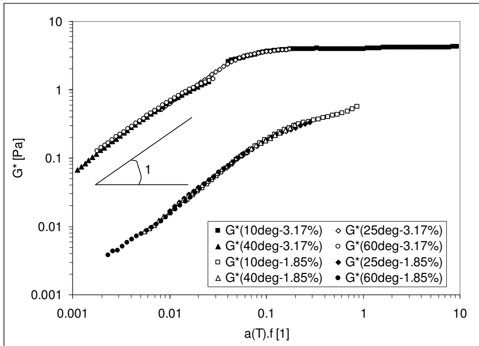
Figure 11: Time-temperature superposition of the complex modulus for both concentrations of sludge.
