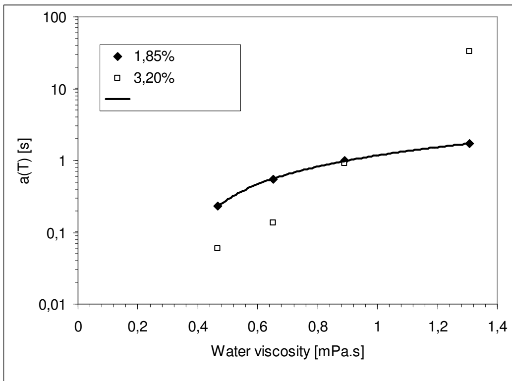
Figure 12: Horizontal shift factor against water viscosity for the 1.85% and 3.2% sludge. The solid line represents a linear model.
