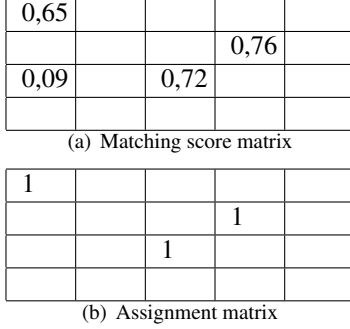
Fig. 4. Example of matching score and assignment matrix
