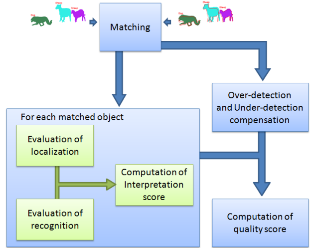
Fig. 3. Principle of the evaluation process
