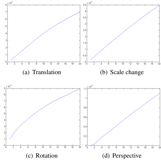
Fig. 6. Results for the localization part
