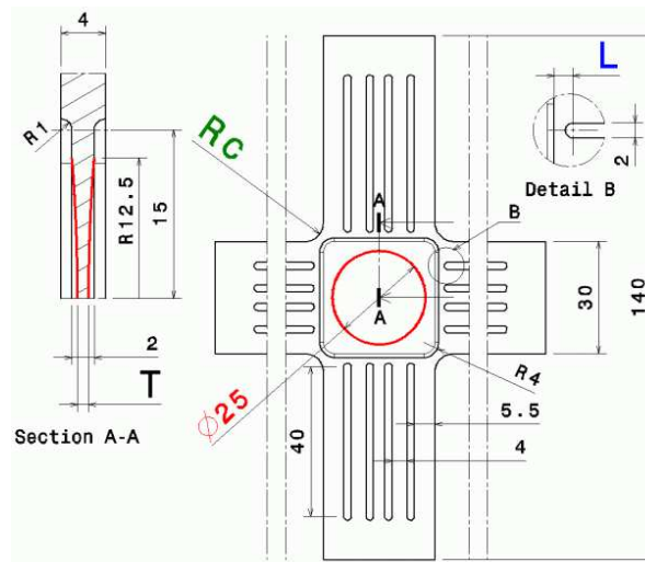
FIGURE 1. Specimen shape.
