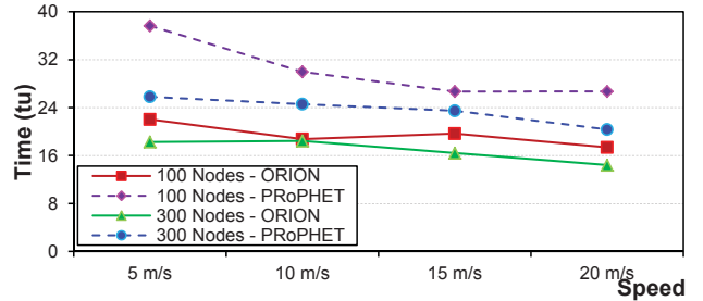
Fig. 10. Average E2E Delay in 100 and 300 nodes topologies with variant speed.
