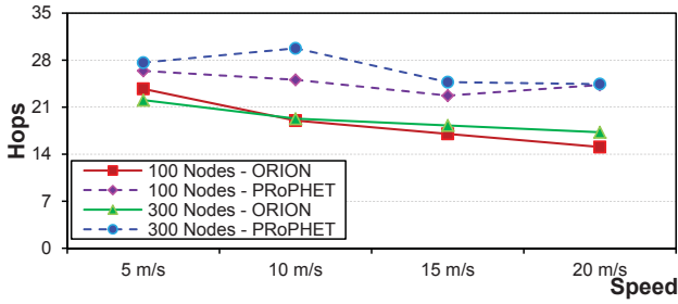
Fig. 7. Average hop count in 100 and 300 nodes topologies with variant speed.
