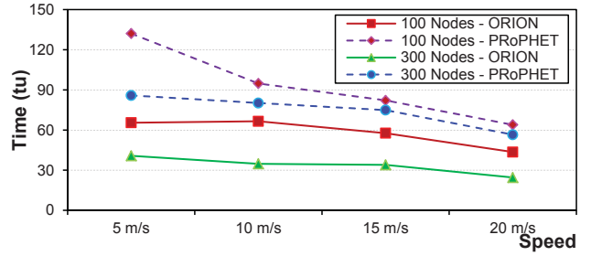
Fig. 9. First Packet Arrival in 100 and 300 nodes topologies with variant speed.
