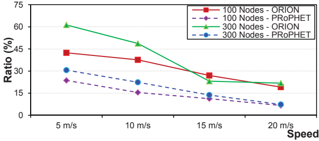
Fig. 8. Packet Success Ratio in 100 and 300 nodes topologies with variant speed.
