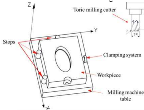
Fig. 2. Defining of action axis of the tool – Machining assembly
