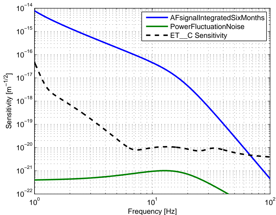
FIG. 4: Expected signal when using ET optimized for low frequency.
