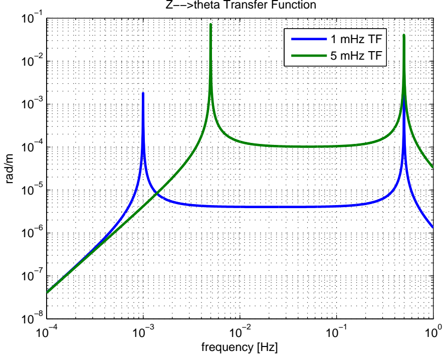
FIG. 6: Transfer function from displacement suspension point to balance’s tilt for 1mHz and 5 mHz resonance frequency. The coupling depends on the resonant frequency.
