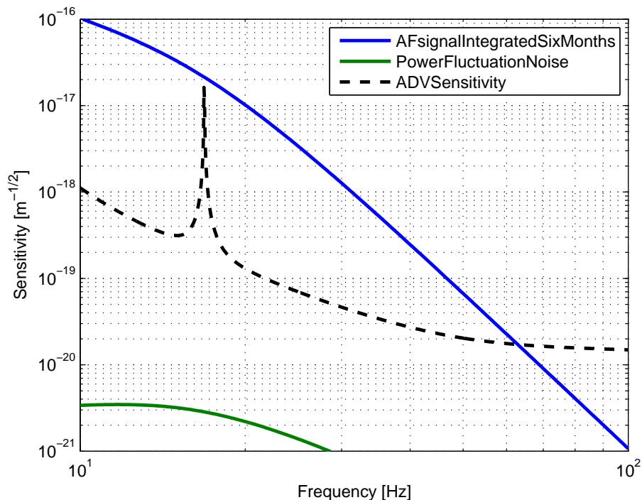
FIG. 3: Expected signal for the YBCO actuator described in the previous Section.
