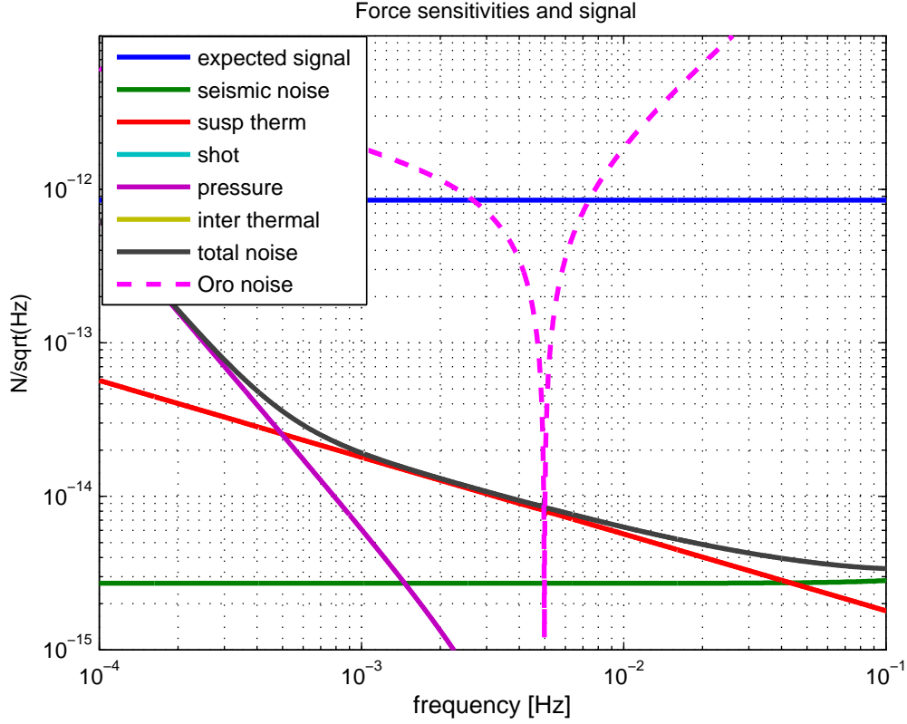
FIG. 8: Force signal and noises. The dashed line describes the noise of an optical lever detection system.
