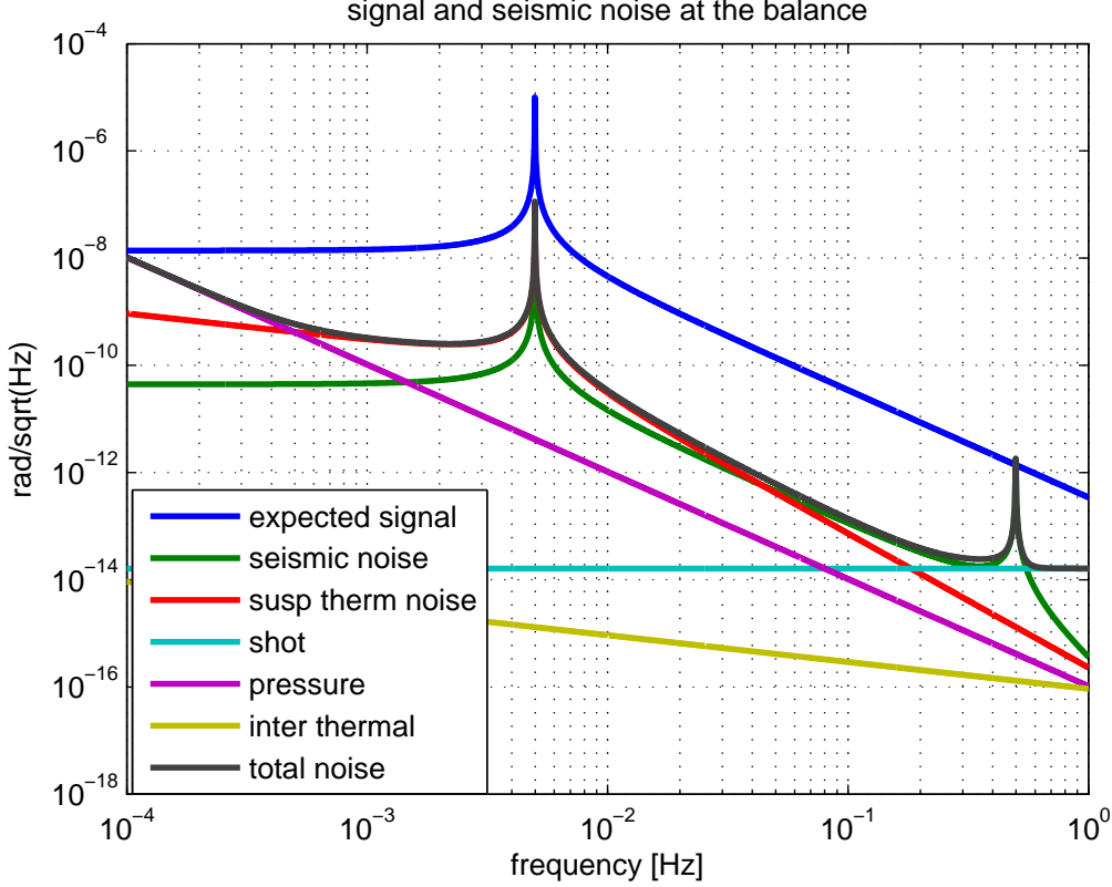
FIG. 7: Expected signal and noises for the balance. In the region of frequencies 5 < f < 100 mHz the signal is about two orders of magnitude above the noise.
