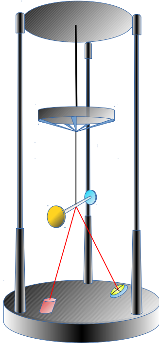
FIG. 5: Sketch of the balance with the optical lever detection read-out. The seismic attenuation chain is composed by the three-legs inverted pendulum and by the blades-attenuation element. The read-out is composed by a laser beam that reflects on the bottom of the bar and impinges on a quadrant photodiode.
