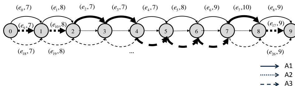
Figure 3: Reduction from 3-PARTITION problem with k = 3
