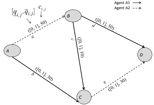
Figure 1: Problem description of example 1
