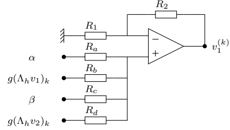
Fig. 5. Analog computation of the k -th equation (17).
