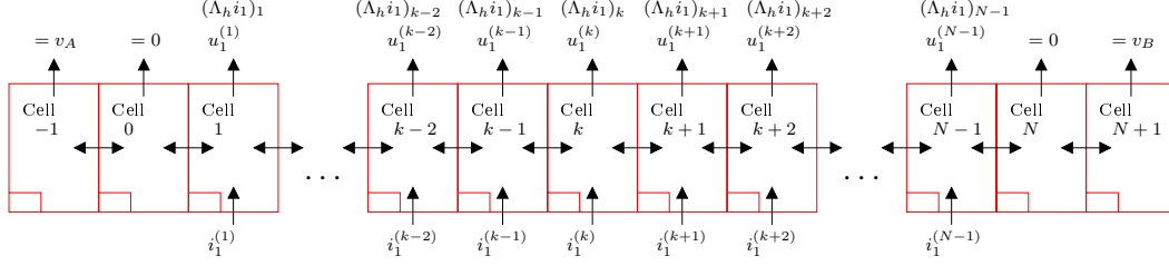
Fig. 2. Analog computation of \Lambda_h v_1 .
