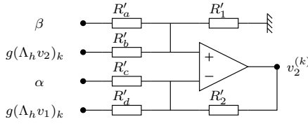
Fig. 6. Analog computation of the k -th equation (18).
