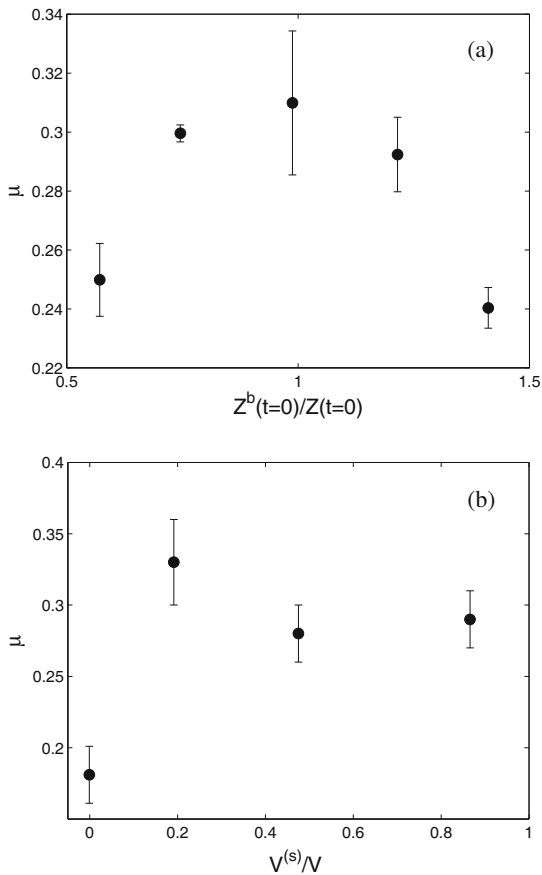
Fig. 14. Effective friction coefficient \mu obtained from eq. (7) as a function of (a) Z^b(t=0)/Z(t=0) and (b) V^{(s)}/V .
