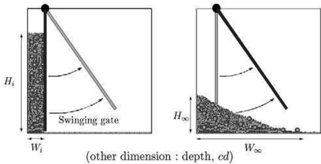
Fig. 1. Experimental configuration.
