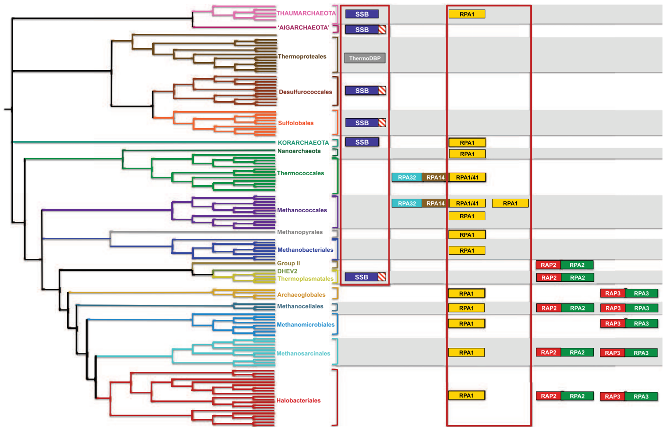
Fig. 5. —Taxonomic distribution and diversity of archaeal SSB and RPA homologs plus the associated proteins (RAP2 and RAP3). ThermoDBP, the proposed replacement for the native SSB of Thermoproteales, is shown in gray. See text for details.
