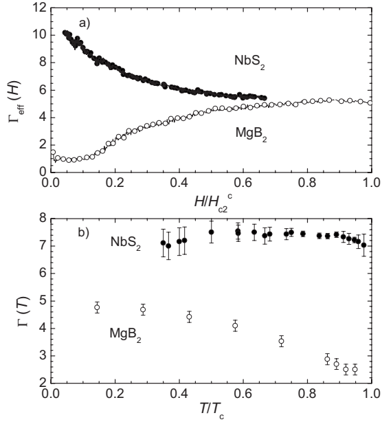
FIG. 4. Anisotropy of NbS 2 (full circles) compared to MgB 2 (Refs. 21 and 27) (open circles): (a) field dependence of effective anisotropy defined as the ratio of the fields applied in both principal orientations that correspond to the same \gamma value in Figs. 3(b) and 3(c) (b) temperature dependence of anisotropy \Gamma = H_{c2}^{ab}/H_{c2}^c .
