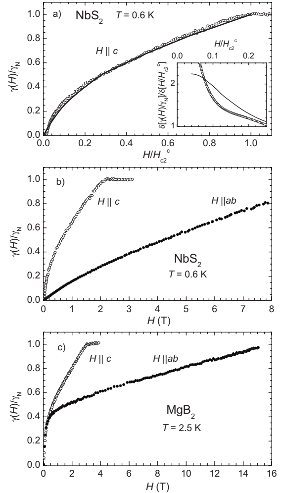
FIG. 3. (a) Open circles: normalized Sommerfeld coefficient \gamma as a function of magnetic field perpendicular to the ab planes of \text{NbS}_2 . Line: model accounting for highly anisotropic gap with \alpha = 0.5 (Ref. 20). Inset is the derivative of the corresponding curves from the main panel: open circles—of the measured data, line—of the model. (b) and (c) \gamma/\gamma_n for both orientations of the magnetic field in \text{NbS}_2 and \text{MgB}_2 (Ref. 21), respectively.
