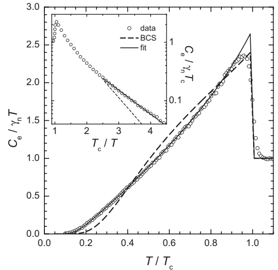
FIG. 2. Open circles: electronic specific heat of \text{NbS}_2 in zero magnetic field extended down to 0.6 K. Dashed line: BCS single-gap weak-coupling case. Solid line: two-gap model with 2\Delta_S/k_B T_c = 2.1 , 2\Delta_L/k_B T_c = 4.6 and respective relative contributions \gamma_S/\gamma_n = 0.4 , \gamma_L/\gamma_n = 0.6 . The anisotropic-gap model with anisotropy parameter \alpha = 0.5 and 2\Delta_0/k_B T_c = 3.6 follows essentially the same line. Inset: exponential dependence of the specific heat, the full line represents the best fit of the exponential decay, the dashed line is the behavior expected for a BCS single-gap weak-coupling limit.
