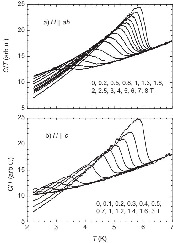
FIG. 1. Total specific heat C/T of \text{NbS}_2 in magnetic field (a) parallel and (b) perpendicular to the ab planes. In both data sets the zero-field measurement is the rightmost curve.
